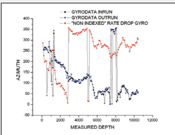
Azimuth vs Measured Depth
