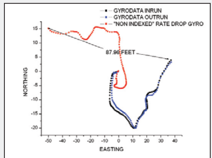
Northings and Eastings
