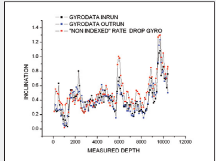
Inclination vs Measured Depth
